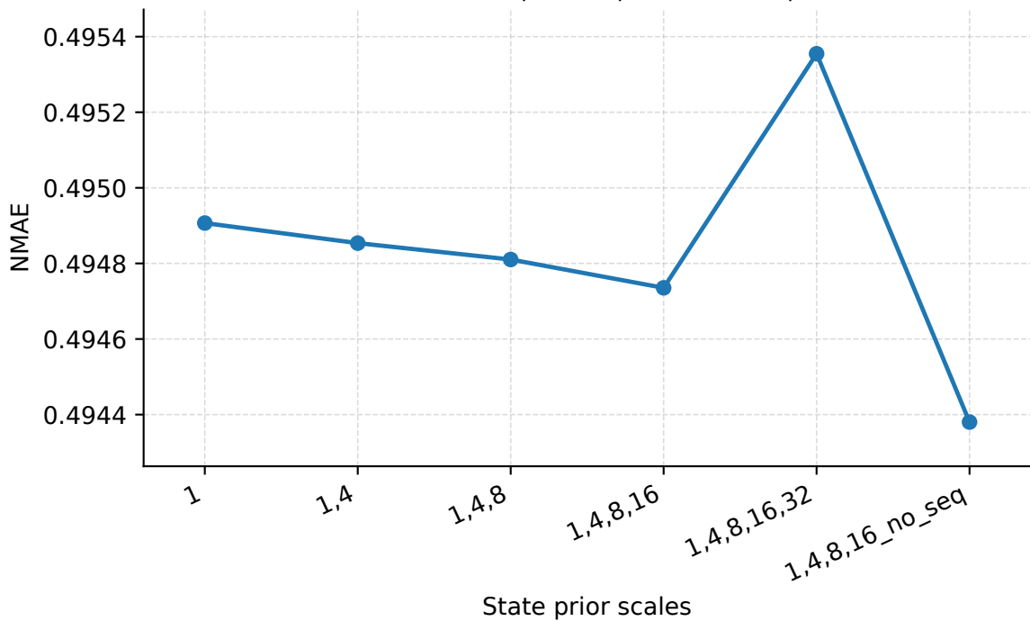
State Prior Scales | Geant | PredLen=20 | NMAE
