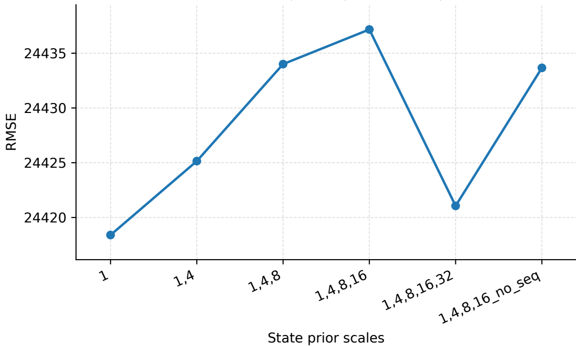
State Prior Scales | Geant | PredLen=20 | RMSE
