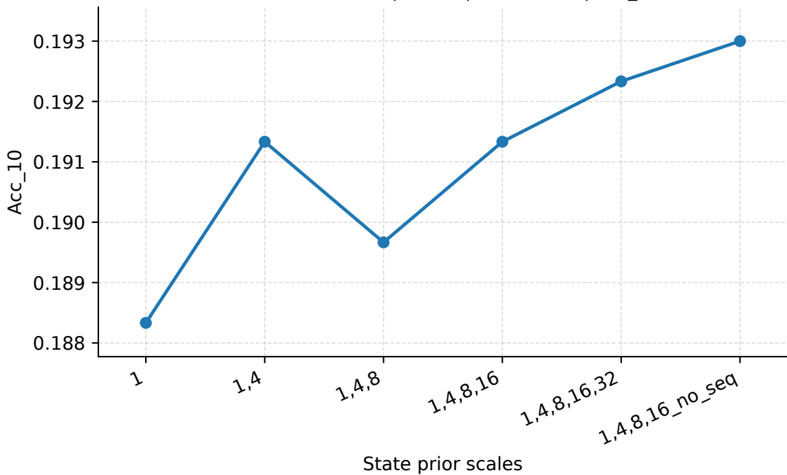
State Prior Scales | Geant | PredLen=5 | Acc_10
