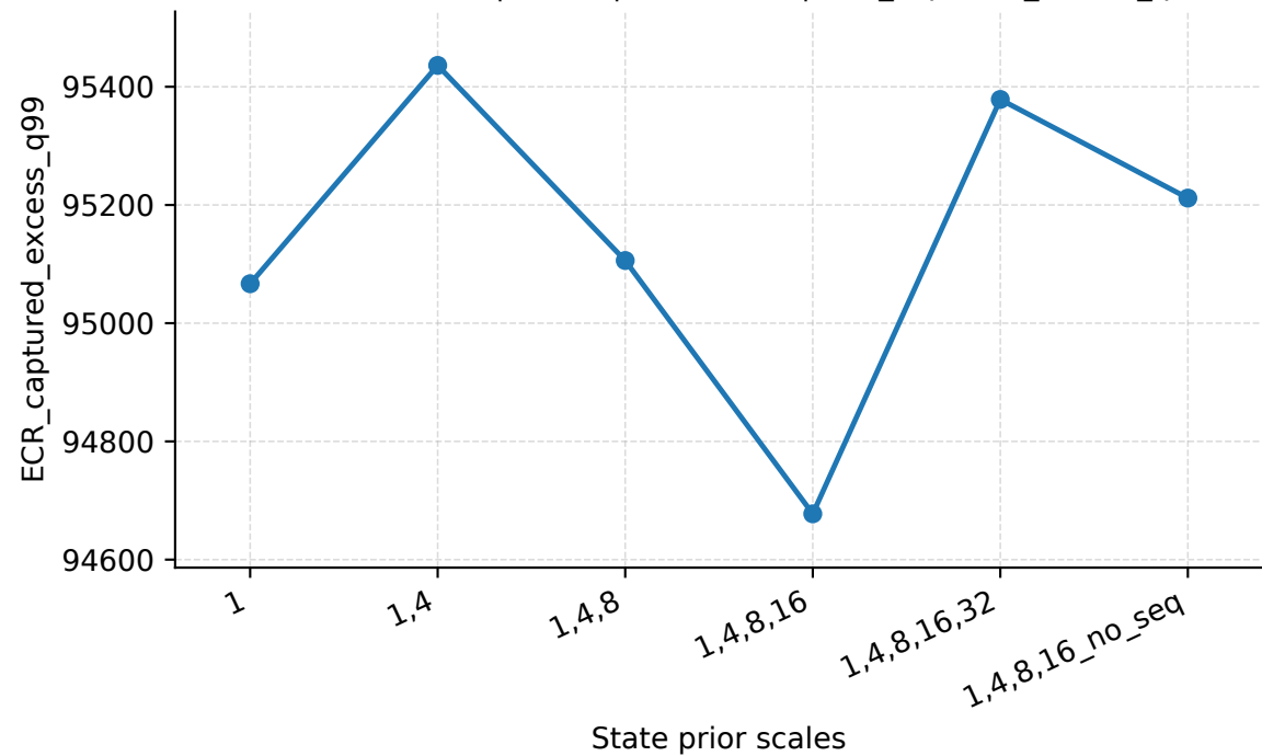
State Prior Scales | Geant | PredLen=5 | ECR_captured_excess_q99
