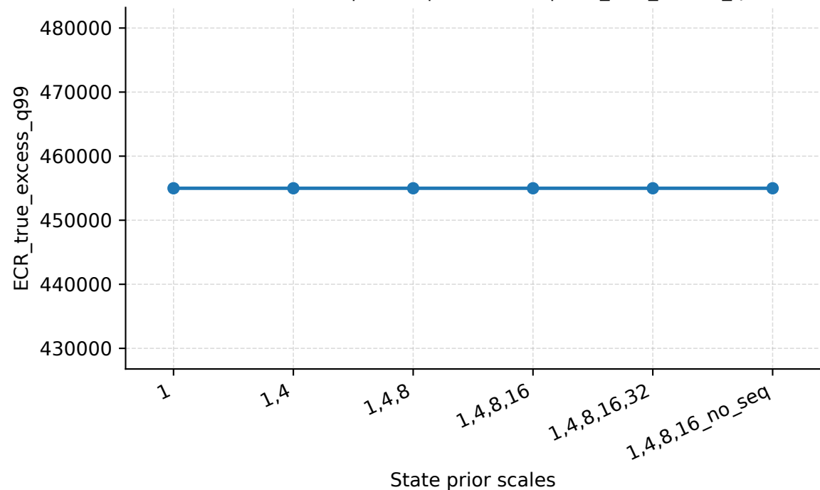
State Prior Scales | Geant | PredLen=5 | ECR_true_excess_q99
