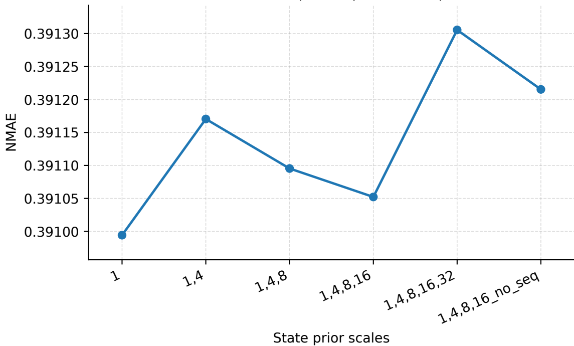
State Prior Scales | Geant | PredLen=5 | NMAE
