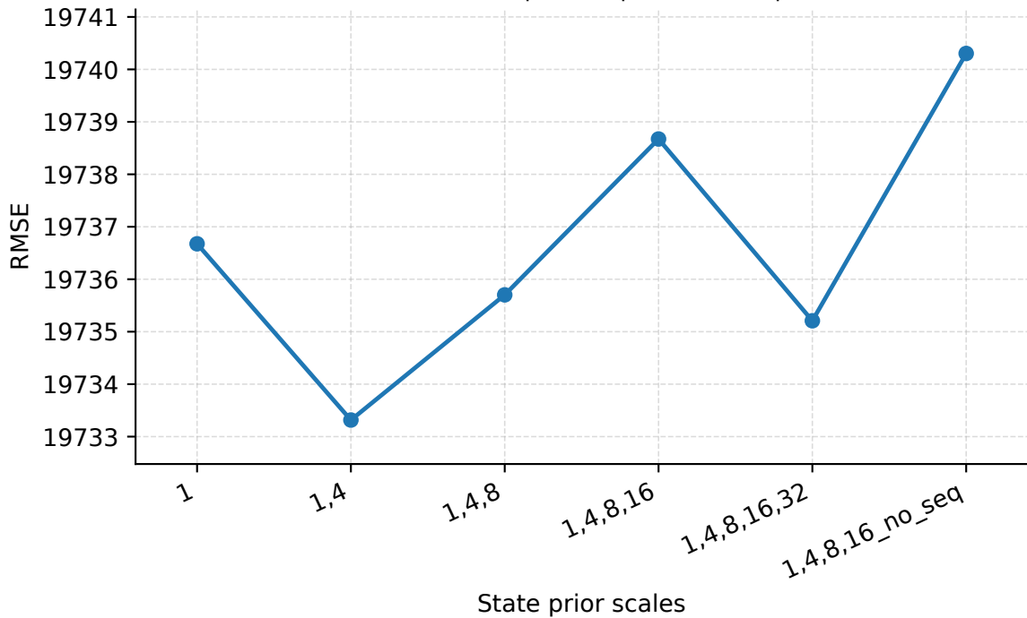
State Prior Scales | Geant | PredLen=5 | RMSE
