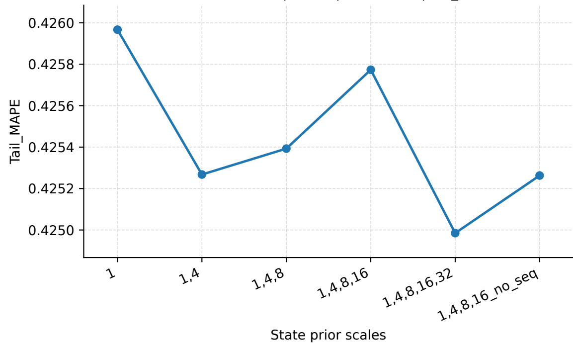
State Prior Scales | Geant | PredLen=5 | Tail_MAPE
