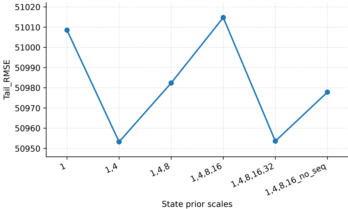
State Prior Scales | Geant | PredLen=5 | Tail_RMSE
