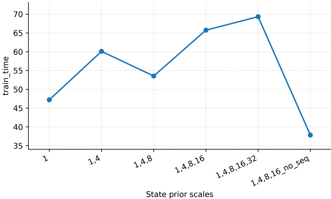
State Prior Scales | Geant | PredLen=5 | train_time
