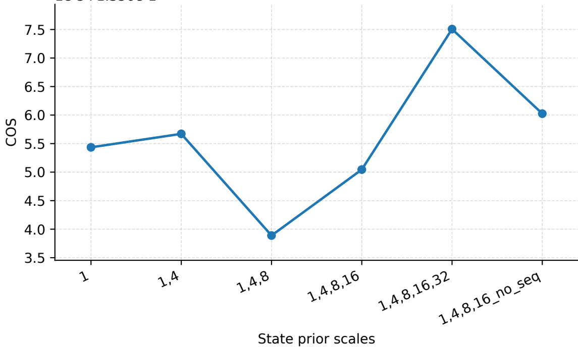
1e-5+1.356e-1 State Prior Scales | Seattle | PredLen=10 | COS
