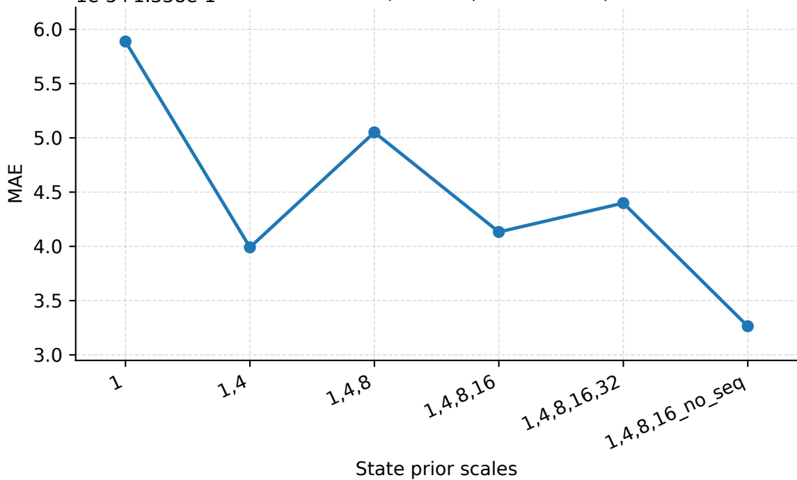
1e-5+1.338e-1 State Prior Scales | Seattle | PredLen=10 | MAE
