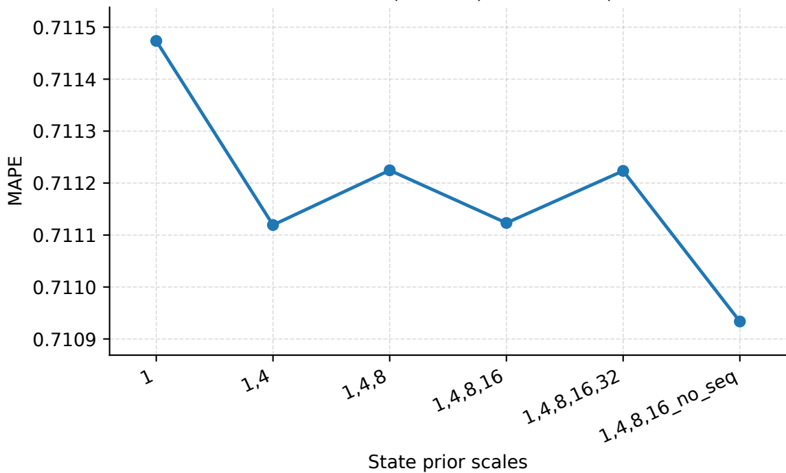
State Prior Scales | Seattle | PredLen=10 | MAPE
