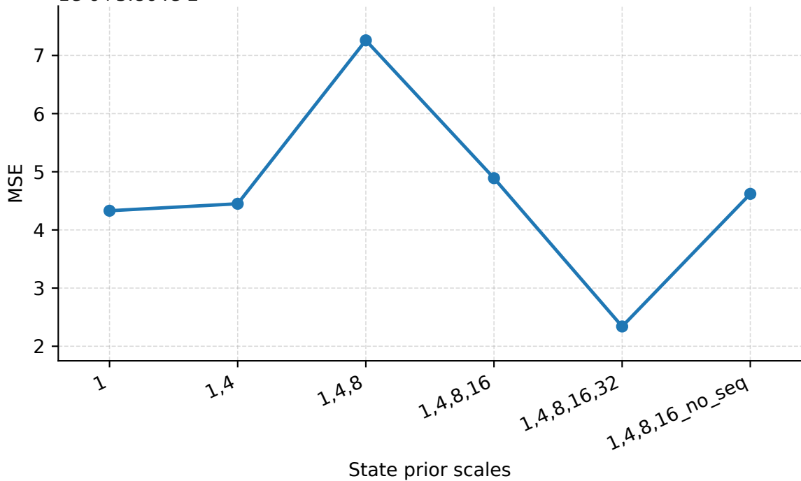
1e-6+3.864e-2 State Prior Scales | Seattle | PredLen=10 | MSE
