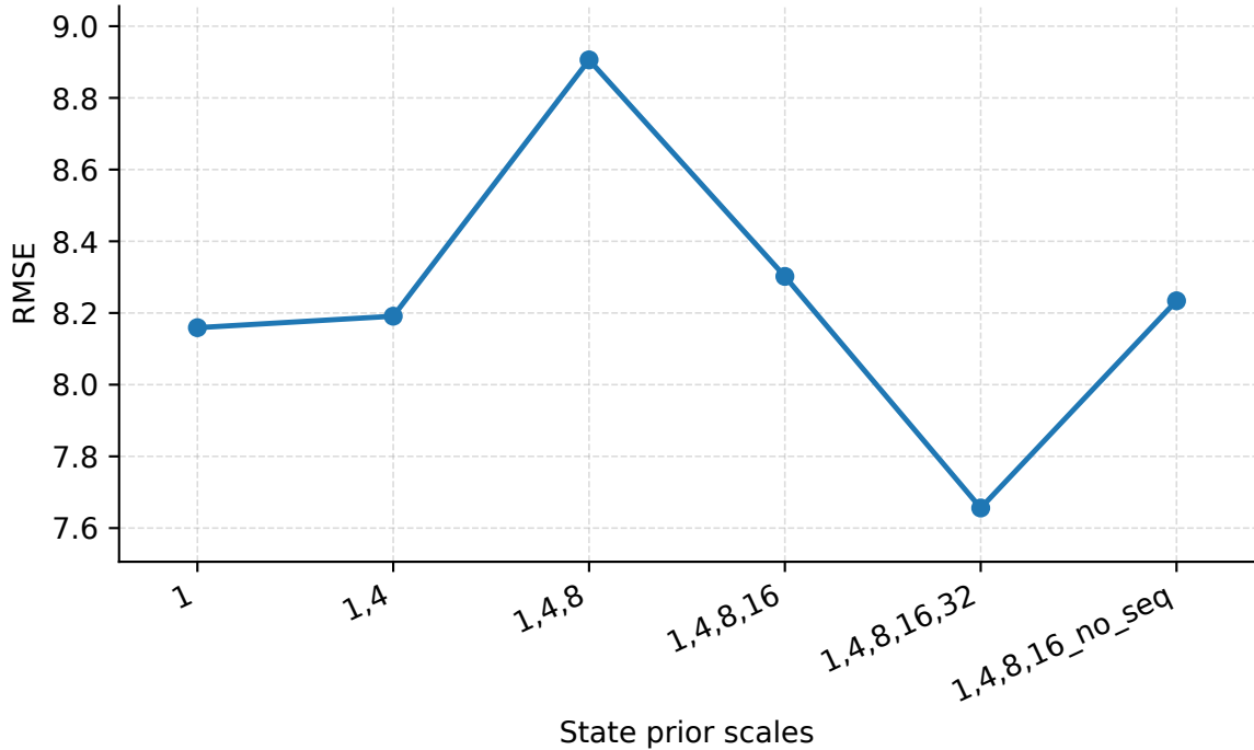
1e-5+1.965e-1 State Prior Scales | Seattle | PredLen=10 | RMSE
