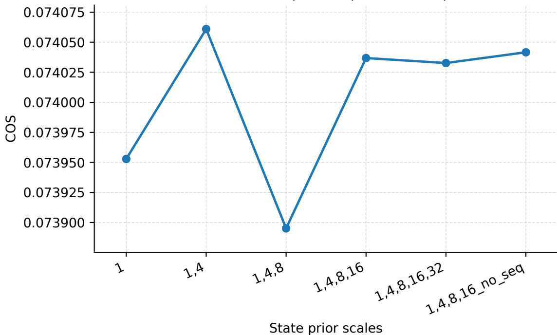
State Prior Scales | Seattle | PredLen=15 | COS
