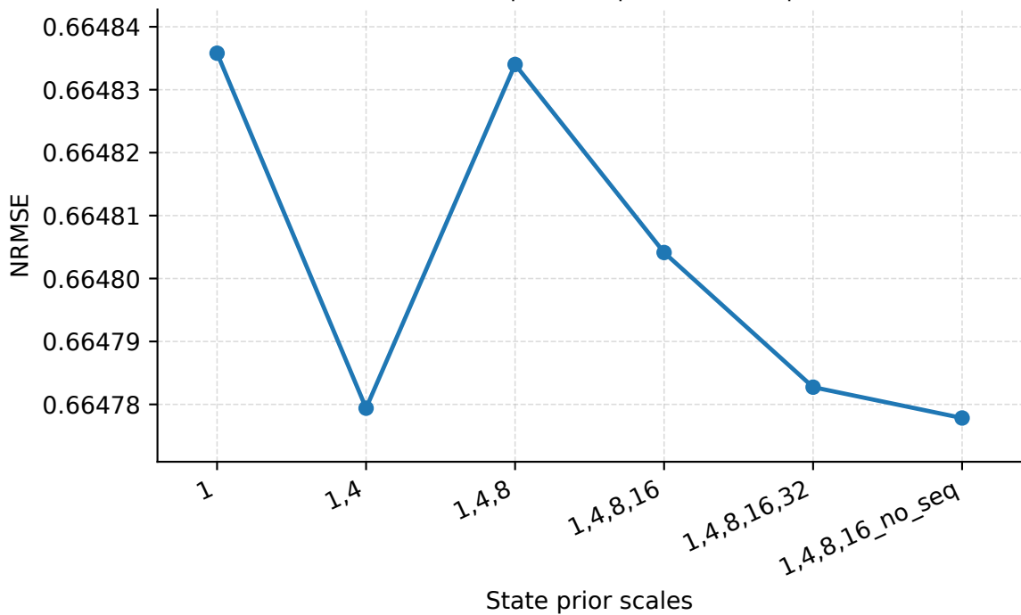
State Prior Scales | Seattle | PredLen=15 | NRMSE
