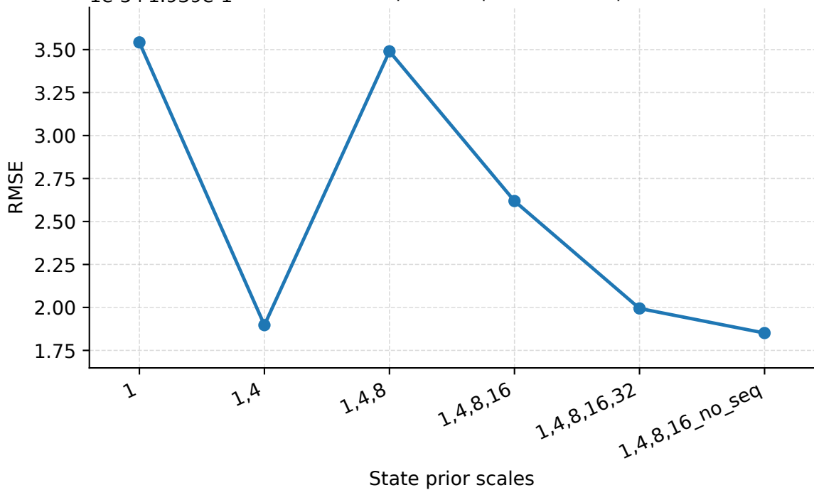
1e-5+1.939e-1 State Prior Scales | Seattle | PredLen=15 | RMSE
