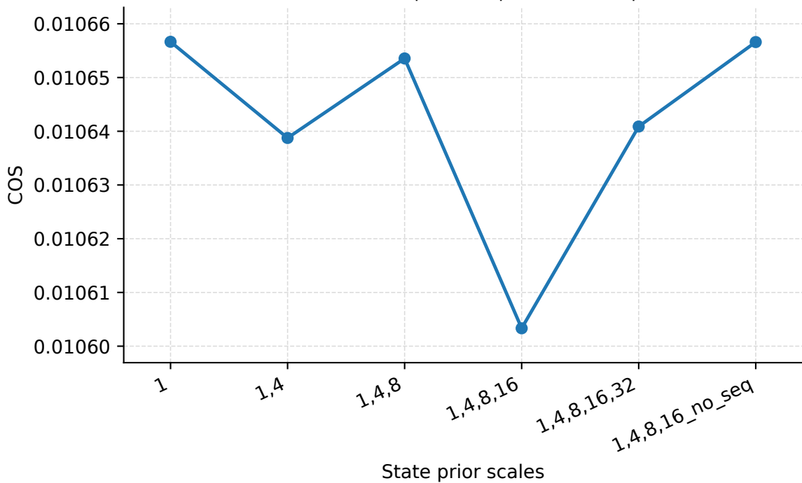
State Prior Scales | Seattle | PredLen=20 | COS
