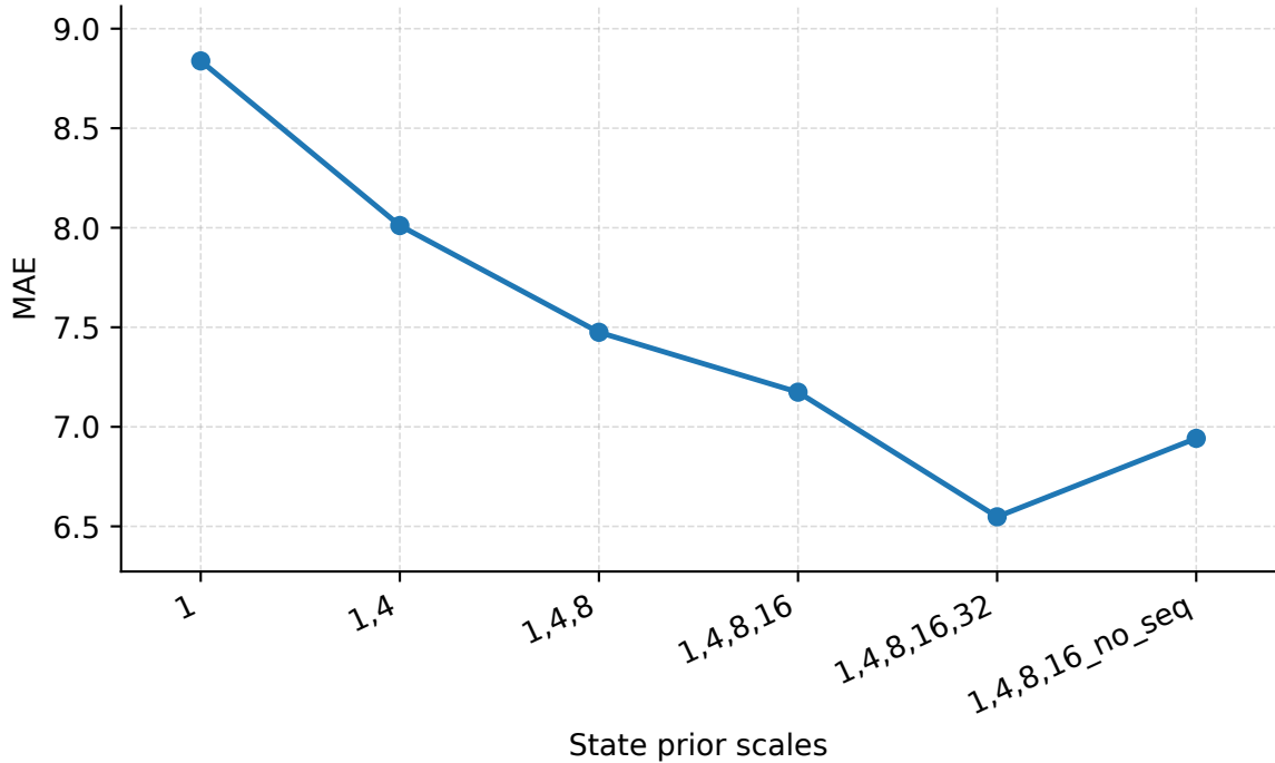
1e-5+1.371e-1 State Prior Scales | Seattle | PredLen=20 | MAE
