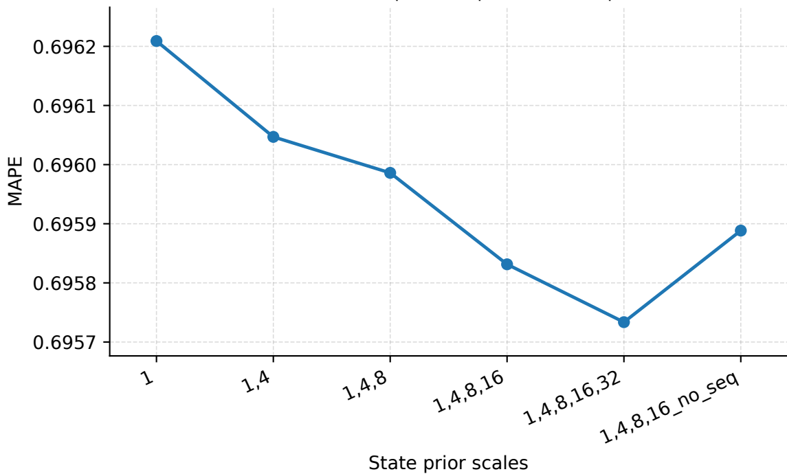
State Prior Scales | Seattle | PredLen=20 | MAPE
