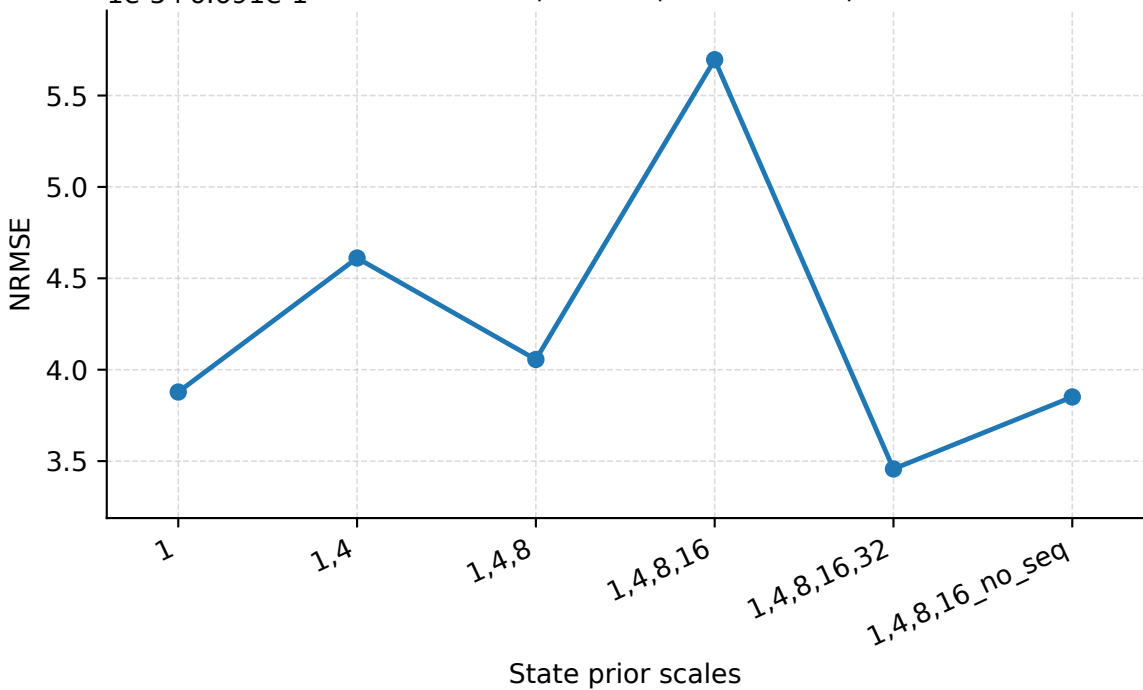
State Prior Scales | Seattle | PredLen=20 | NRMSE
