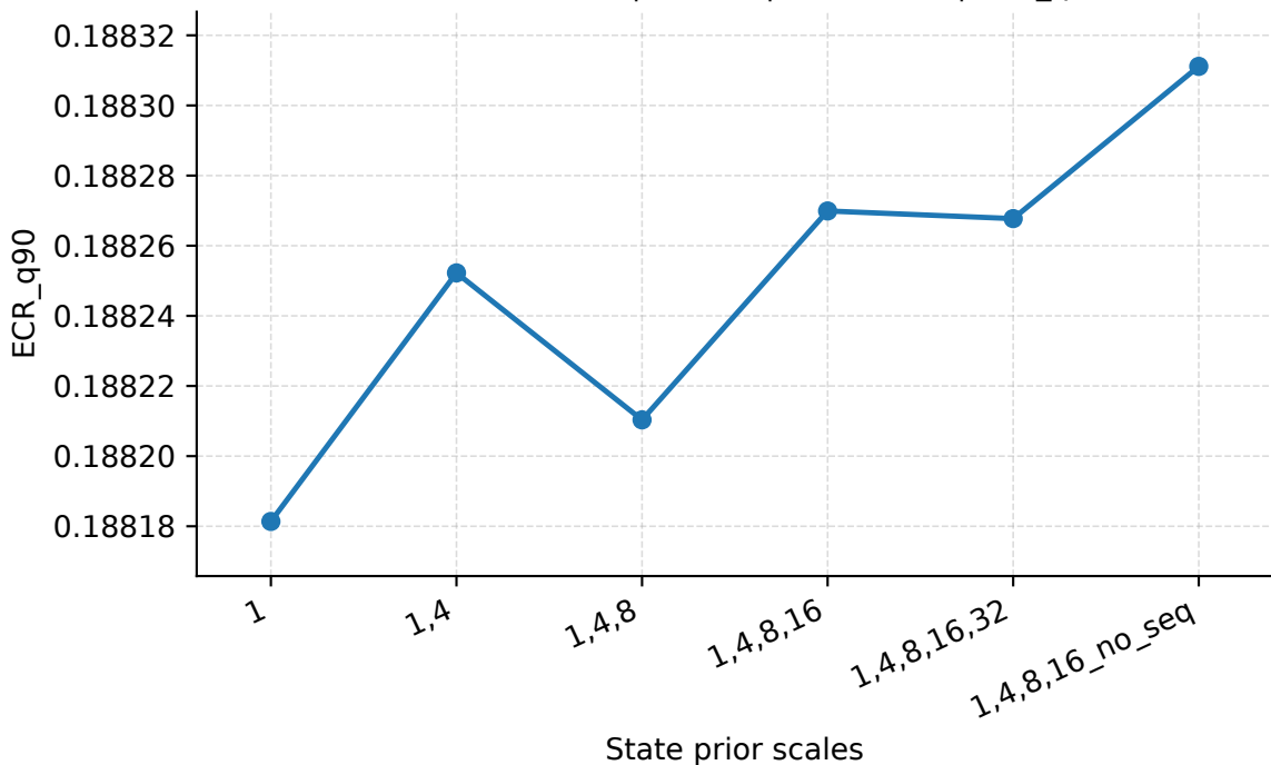
State Prior Scales | Seattle | PredLen=5 | ECR_q90
