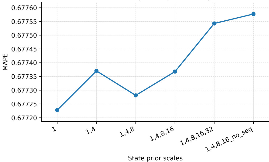
State Prior Scales | Seattle | PredLen=5 | MAPE
