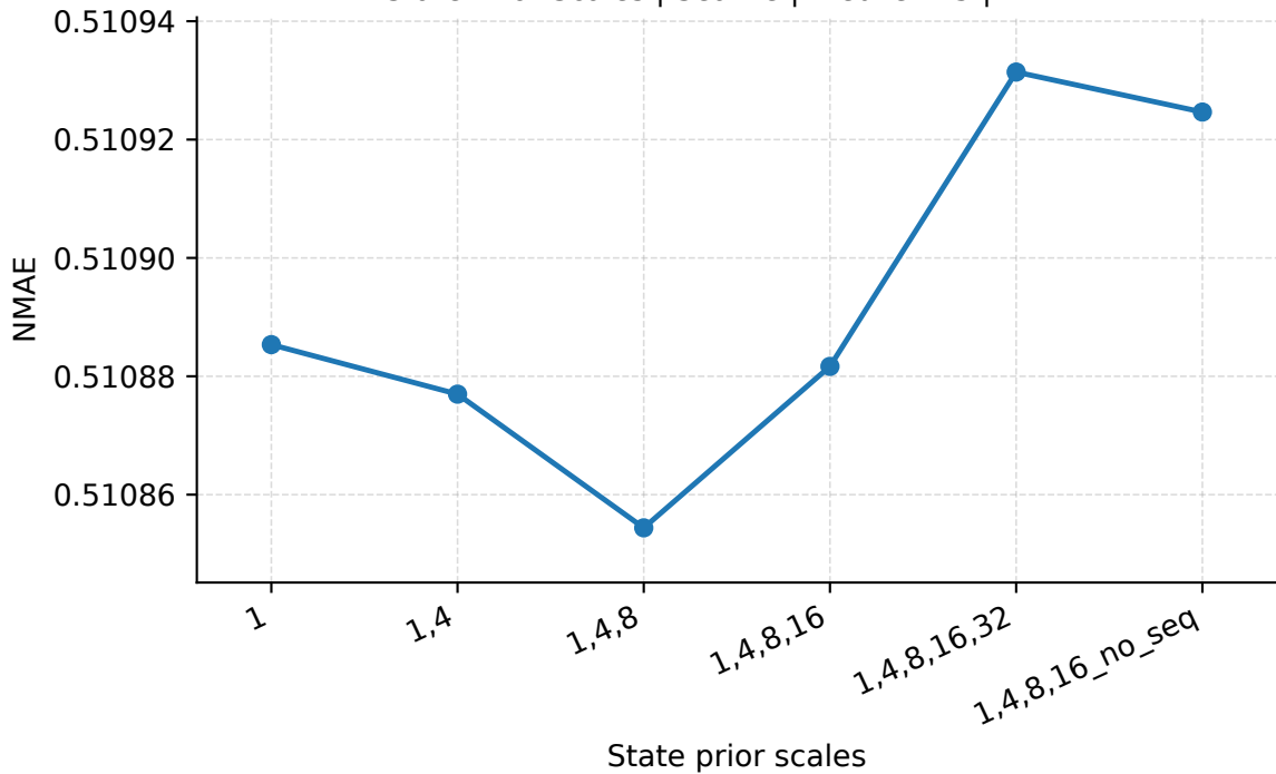
State Prior Scales | Seattle | PredLen=5 | NMAE
