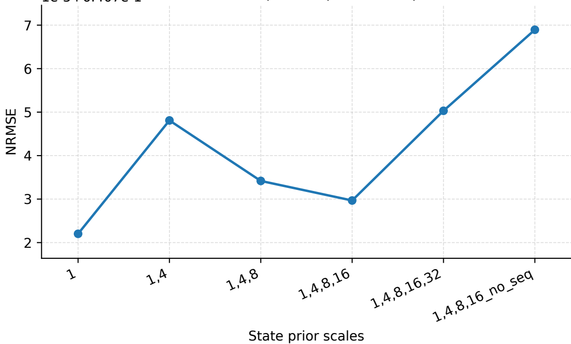
1e-5+6.407e-1 State Prior Scales | Seattle | PredLen=5 | NRMSE
