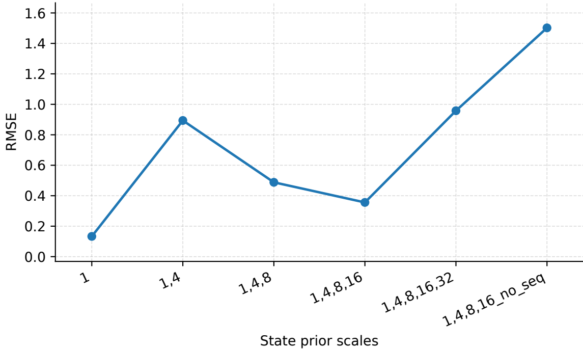
1e-5+1.869e-1 State Prior Scales | Seattle | PredLen=5 | RMSE
