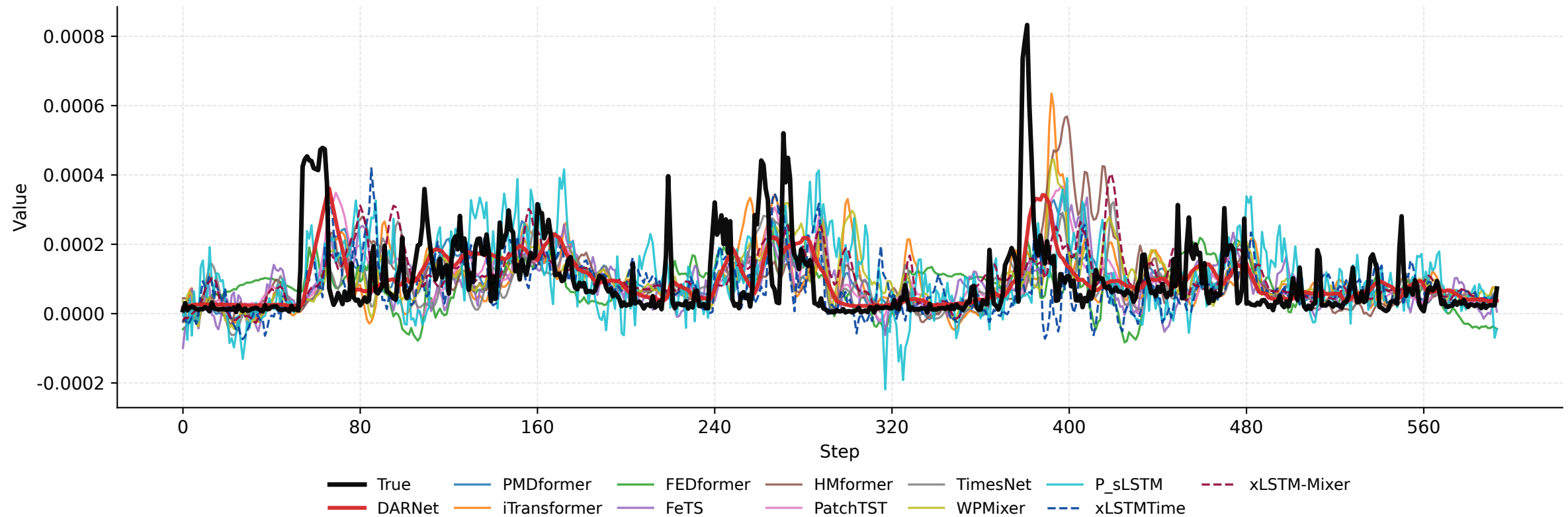
Abilene Prediction Curves (PredLen=10)
