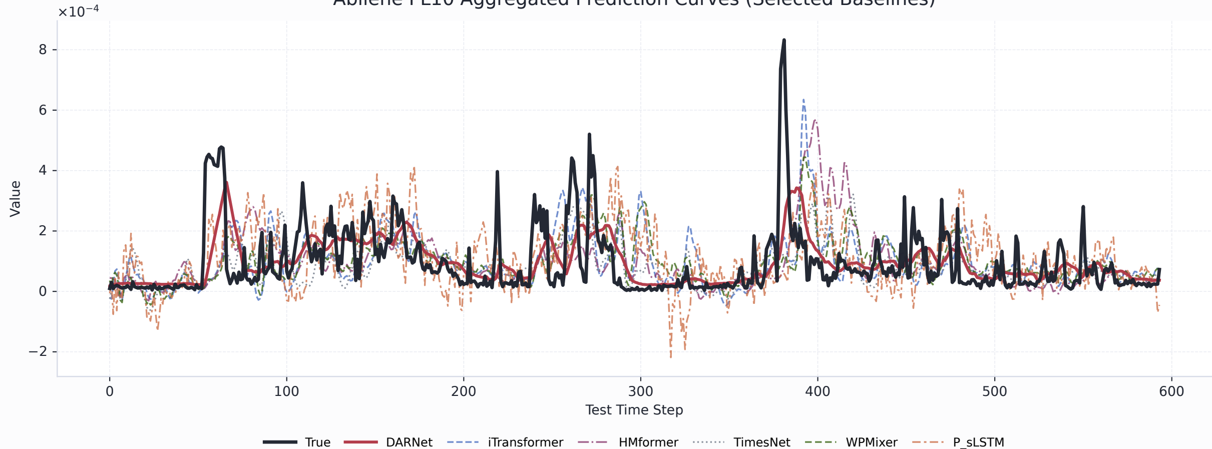
Abilene PL10 Aggregated Prediction Curves (Selected Baselines)
