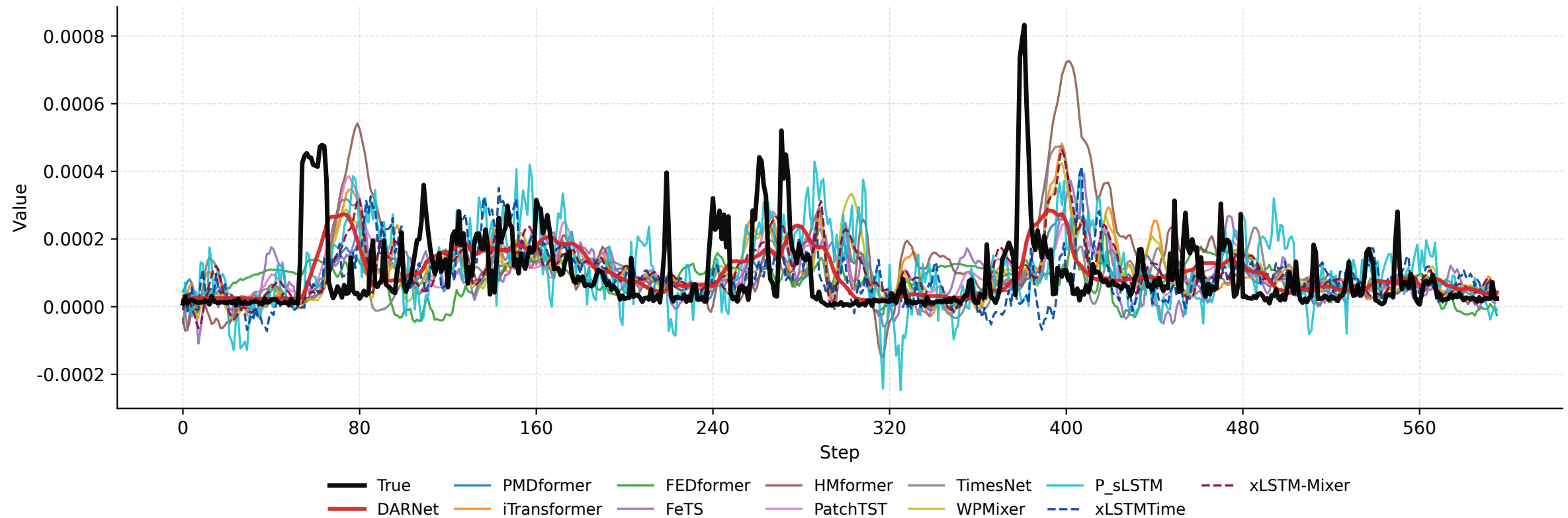
Abilene Prediction Curves (PredLen=20)
