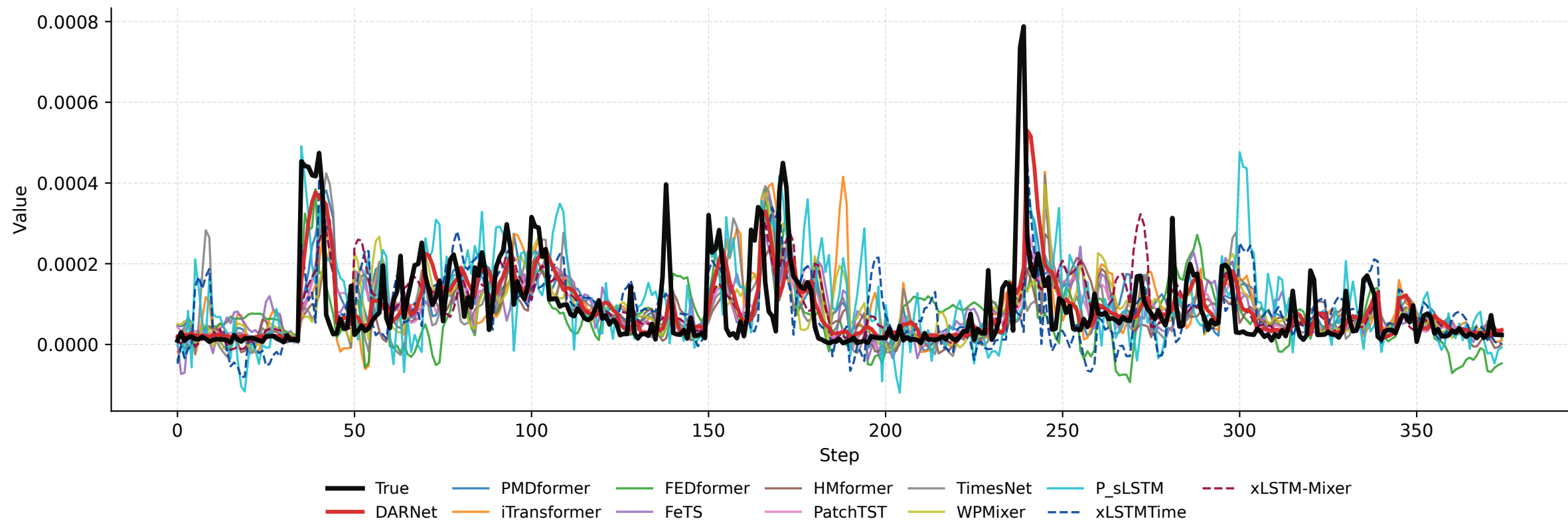
Abilene Prediction Curves (PredLen=5)
