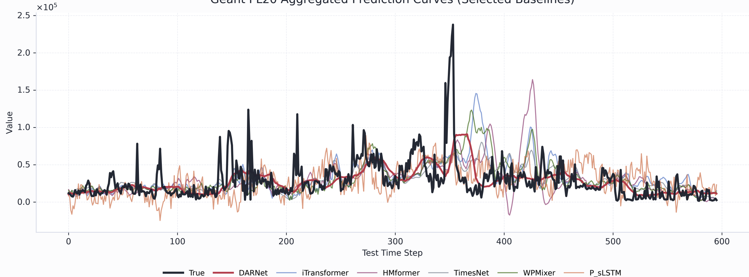
Geant PL20 Aggregated Prediction Curves (Selected Baselines)
