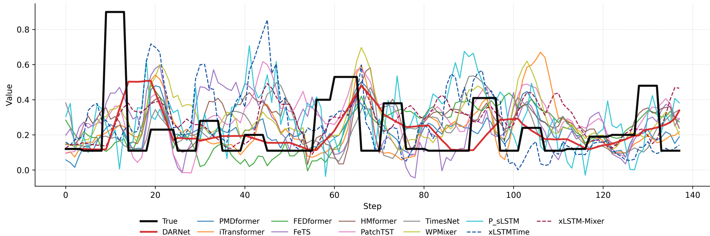
Seattle Prediction Curves (PredLen=10)
