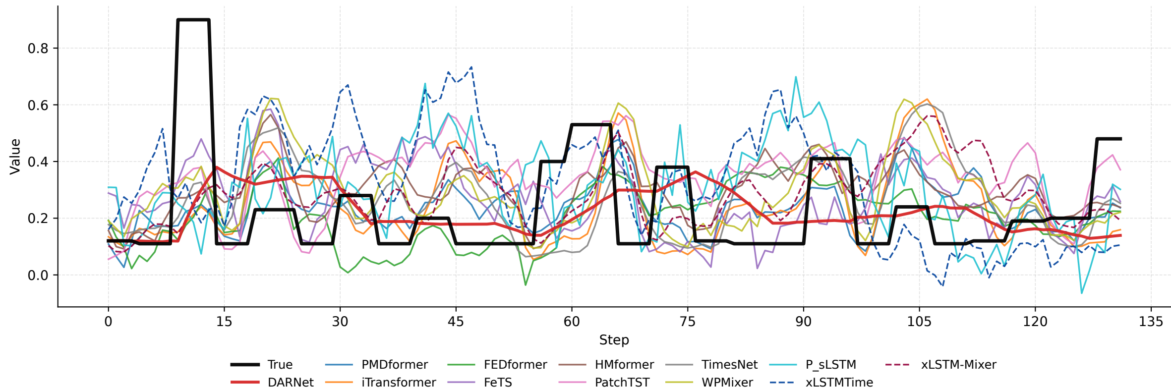
Seattle Prediction Curves (PredLen=20)
