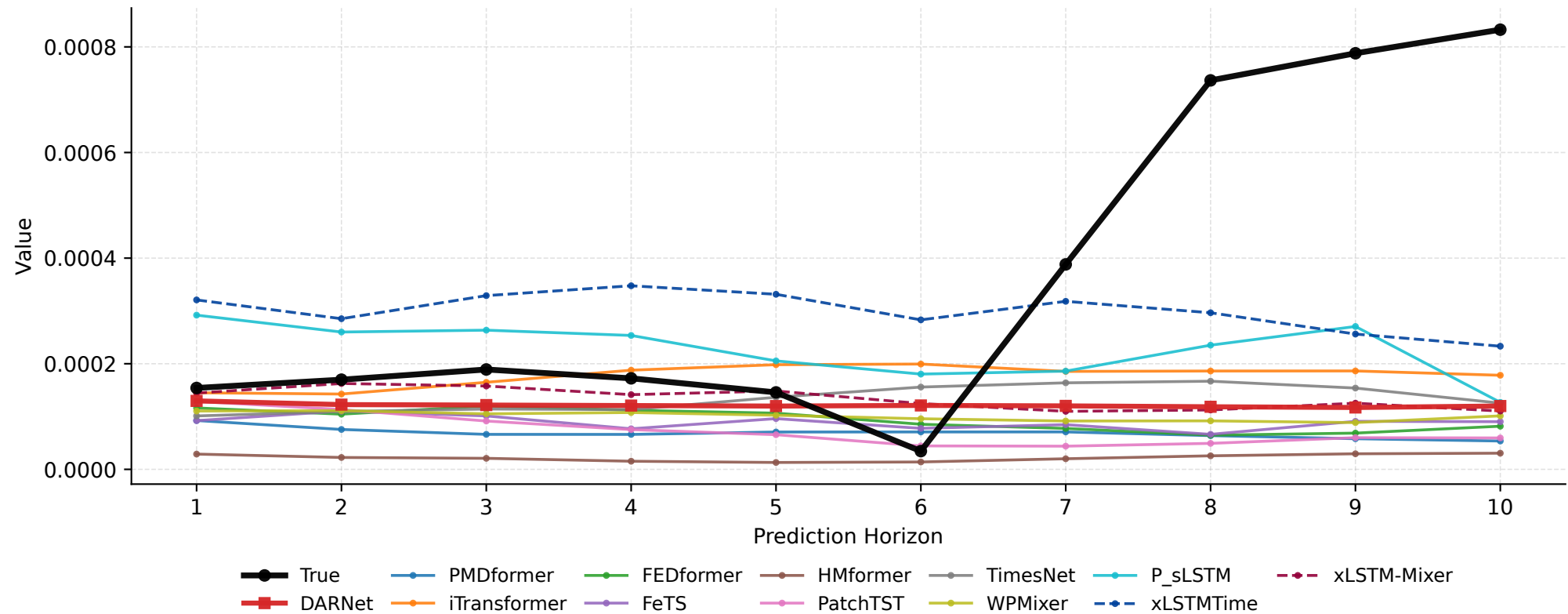
Abilene Forecast Horizon Comparison (PredLen=10, RefWindow=372)
