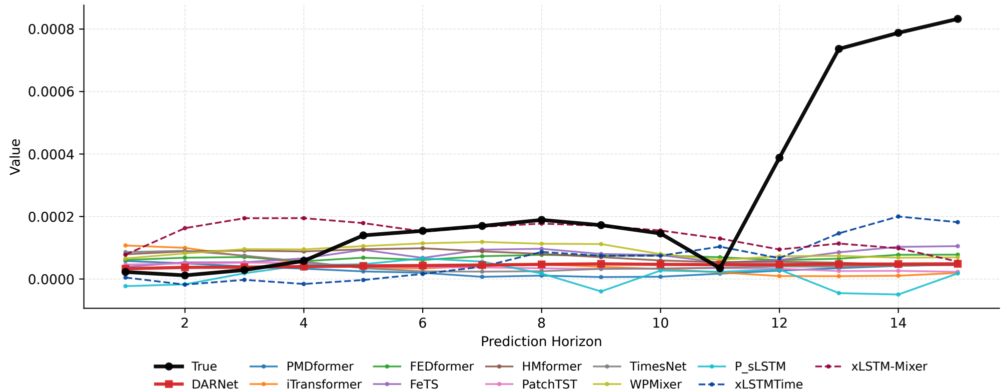
Abilene Forecast Horizon Comparison (PredLen=15, RefWindow=367)
