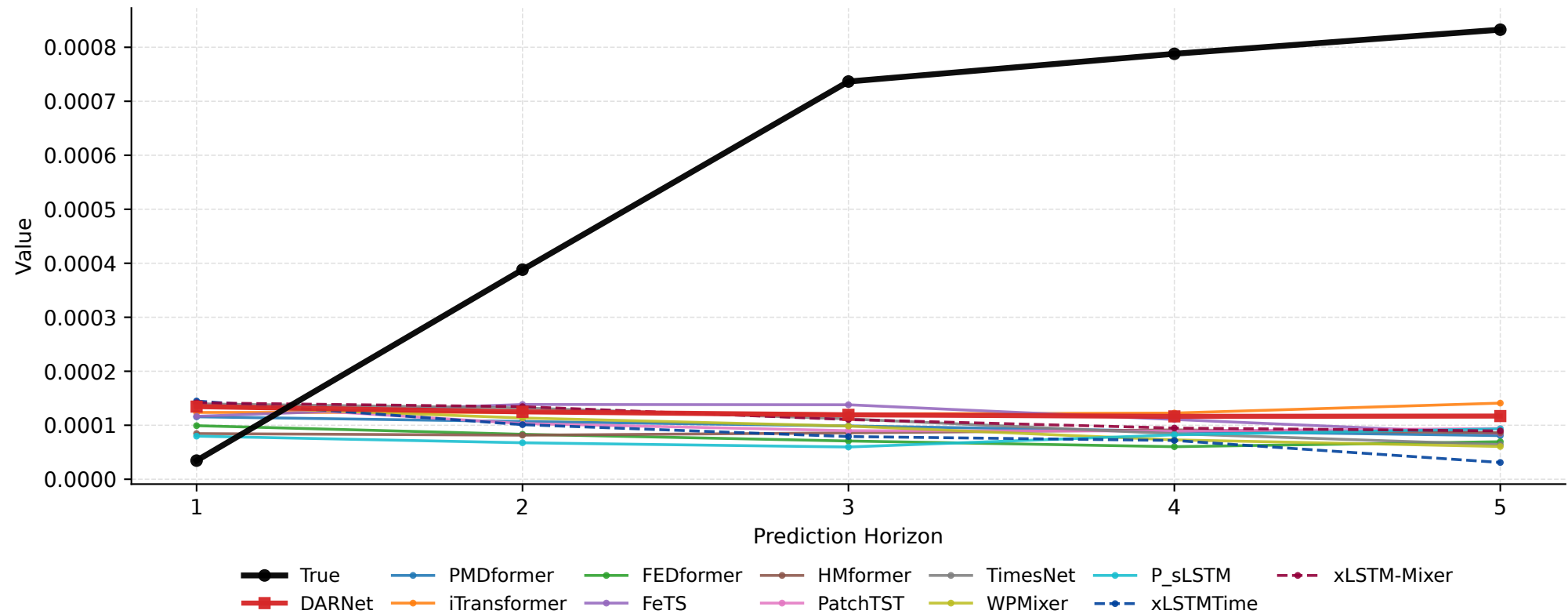
Abilene Forecast Horizon Comparison (PredLen=5, RefWindow=377)
