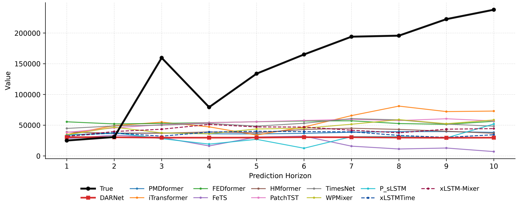
Geant Forecast Horizon Comparison (PredLen=10, RefWindow=344)
