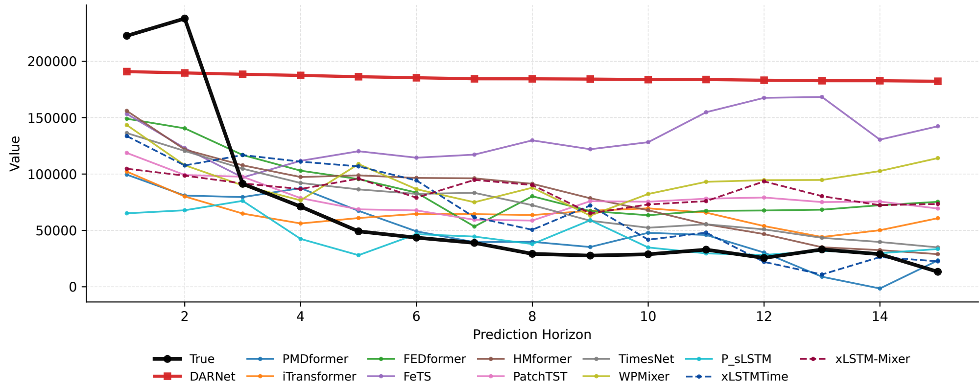
Geant Forecast Horizon Comparison (PredLen=15, RefWindow=352)
