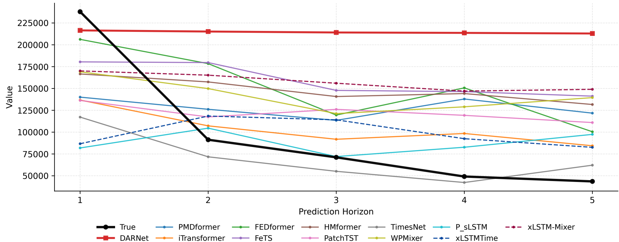
Geant Forecast Horizon Comparison (PredLen=5, RefWindow=353)
