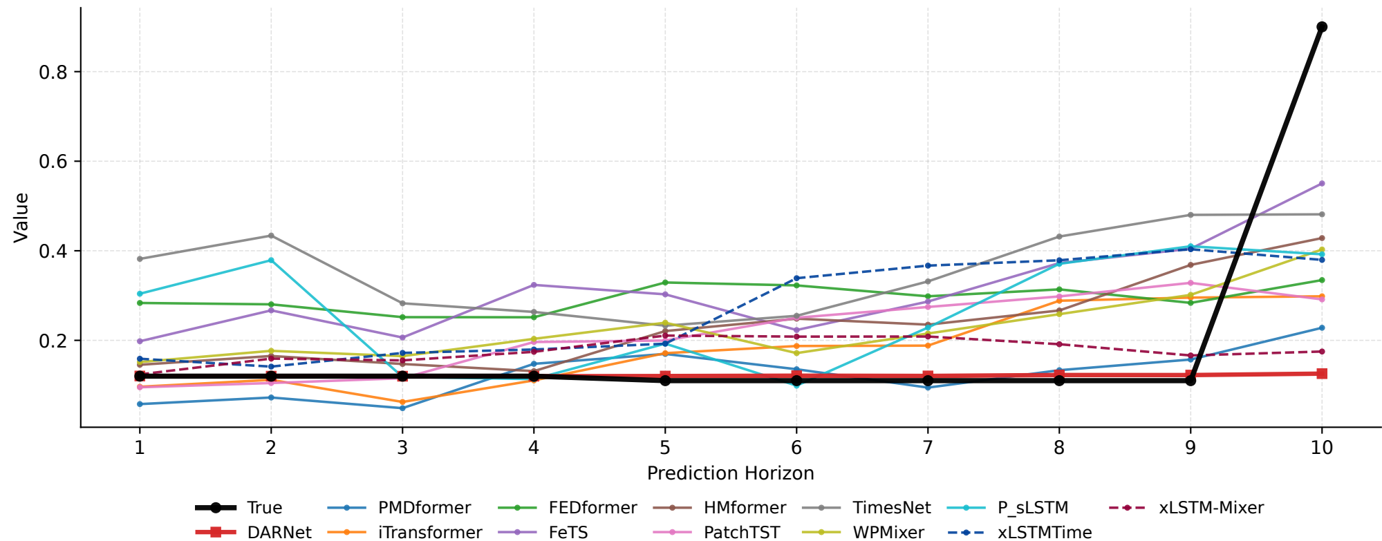
Seattle Forecast Horizon Comparison (PredLen=10, RefWindow=0)
