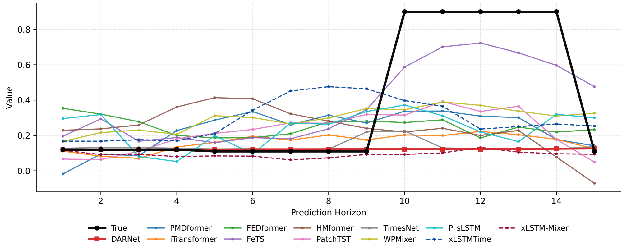
Seattle Forecast Horizon Comparison (PredLen=15, RefWindow=0)
