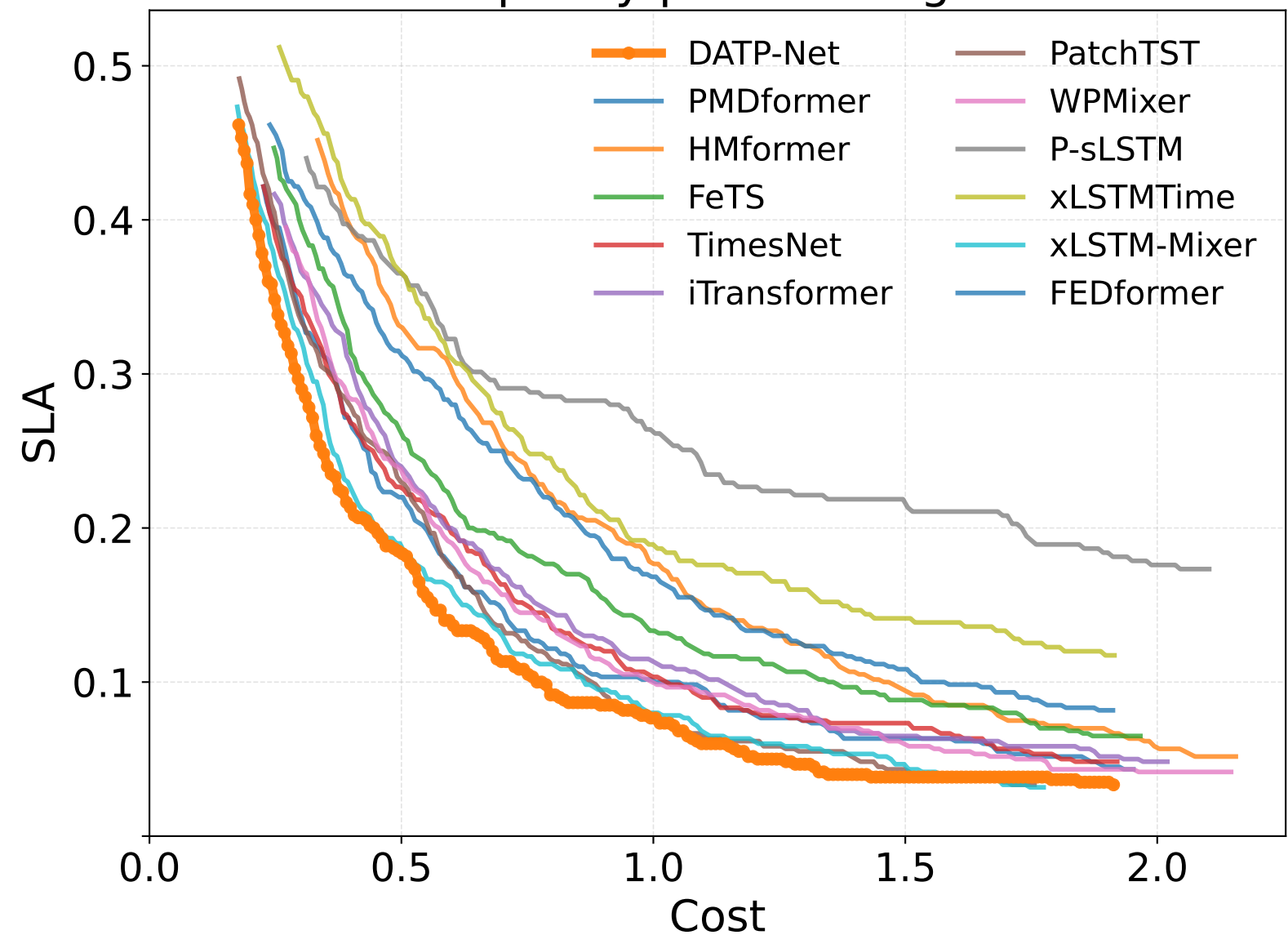
GÉANT capacity provisioning trade-off
