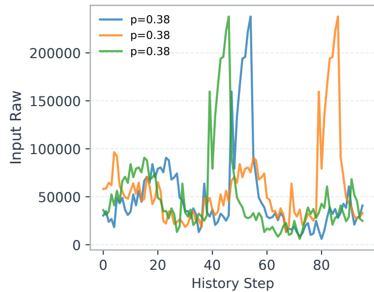
Geant E0
