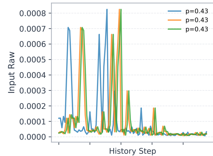
Geant E0
