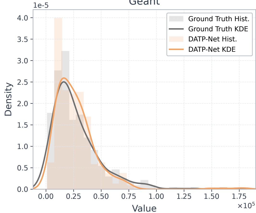
Geant
