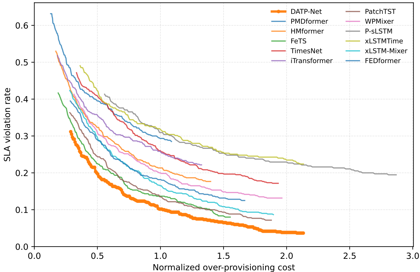
Abilene capacity provisioning trade-off
