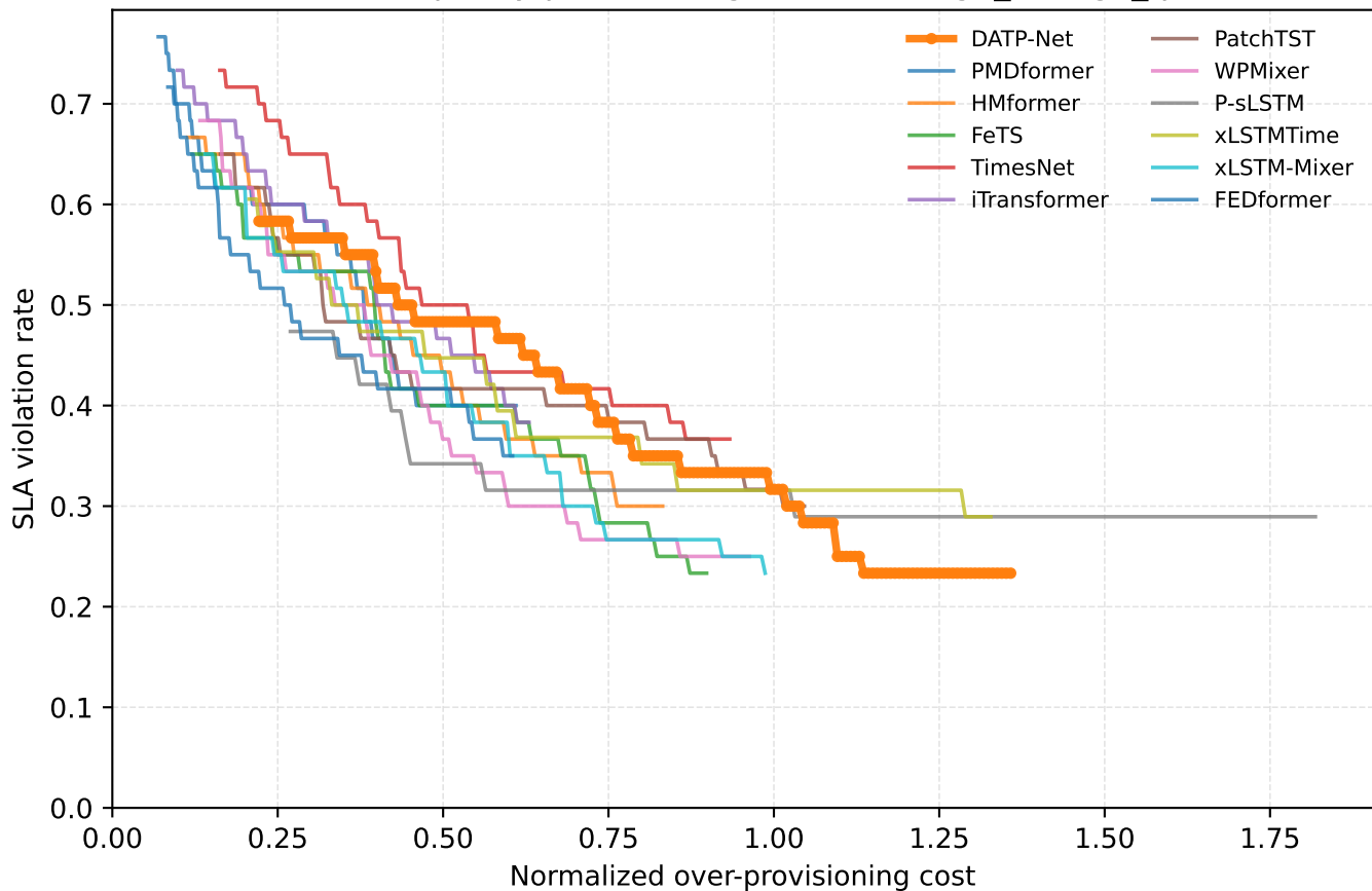
Abilene capacity provisioning trade-off (high_change_q90)
