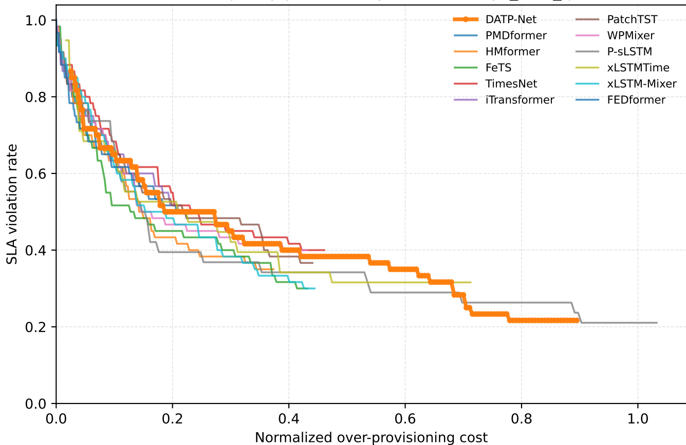
Abilene capacity provisioning trade-off (high_load_q90)
