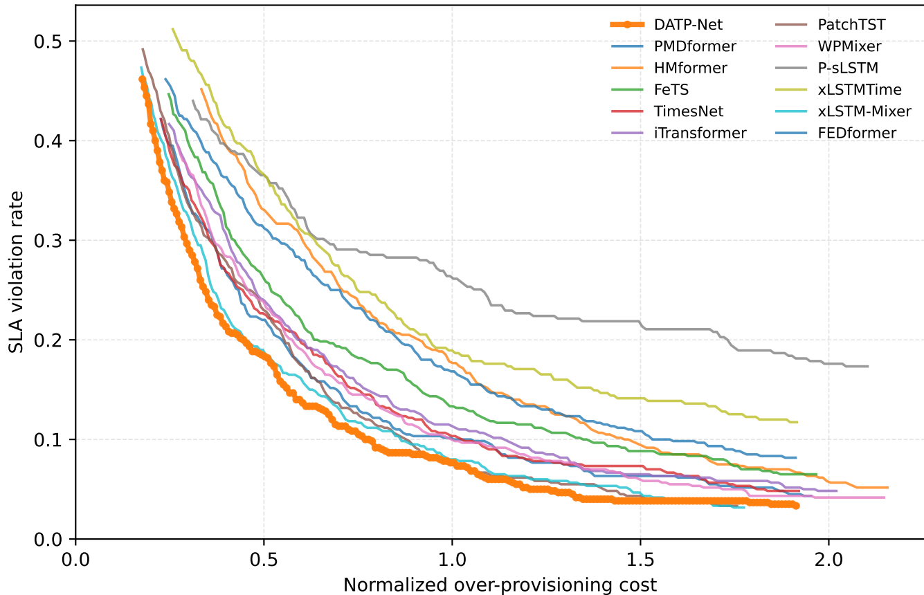
GÉANT capacity provisioning trade-off
