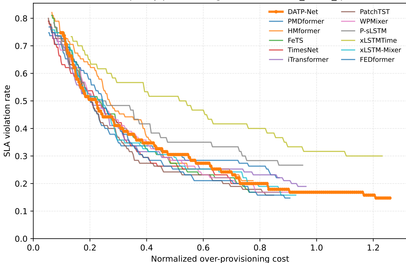
GÉANT capacity provisioning trade-off (burst_union_q90)
